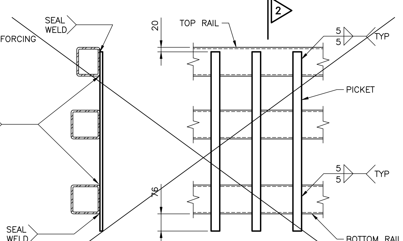
2 PICKET DETAIL (OPTIONAL)
