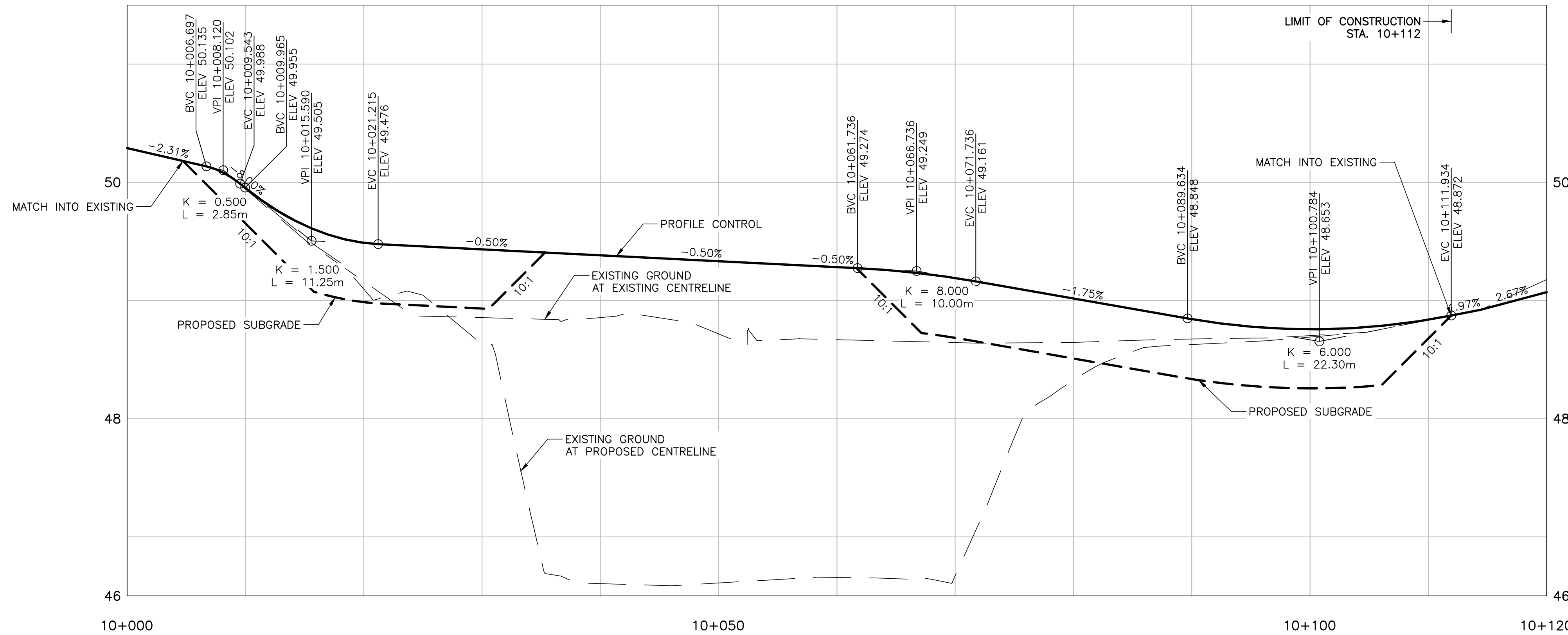
PROFILE OF NEW HAMILTON ISLAND ROAD
