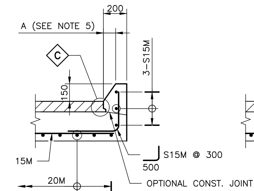
1 SECTION AT CURB SCALE 1:20
