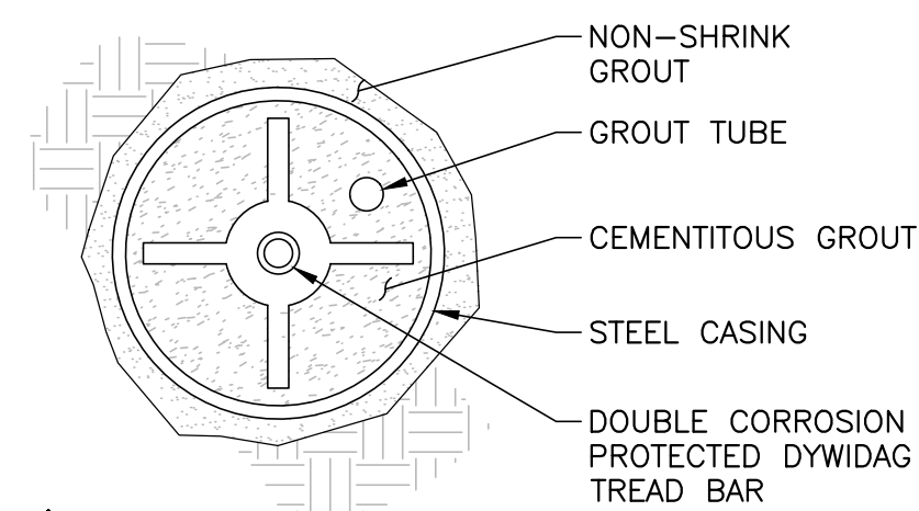
SECTION 3 1:5
