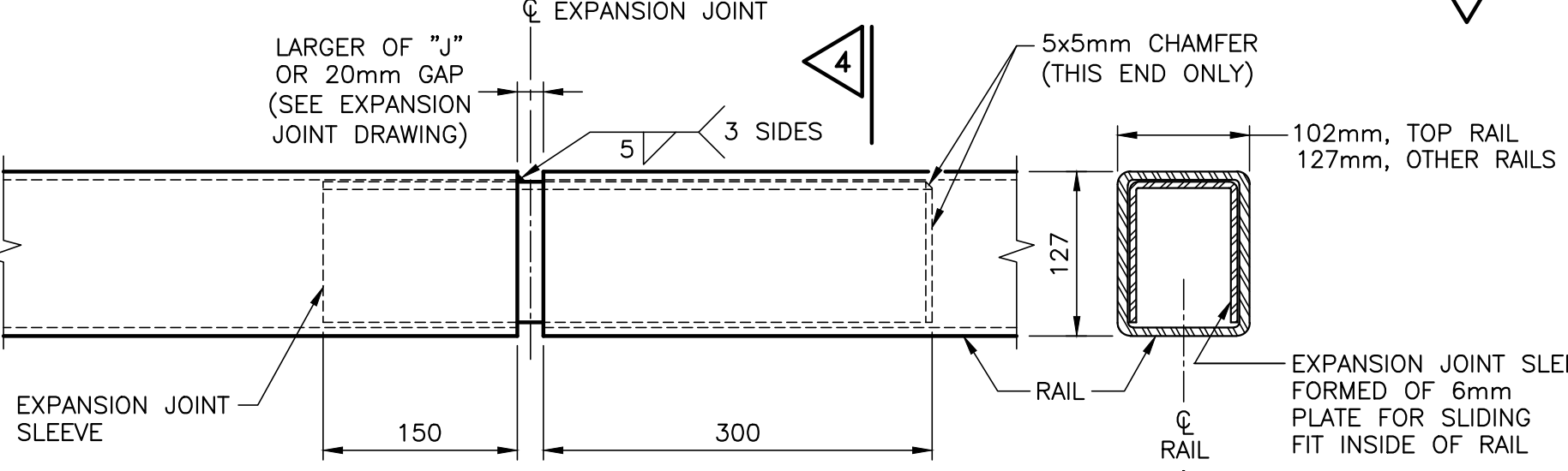
D CONNECTION DETAIL AT EXP. JOINT
