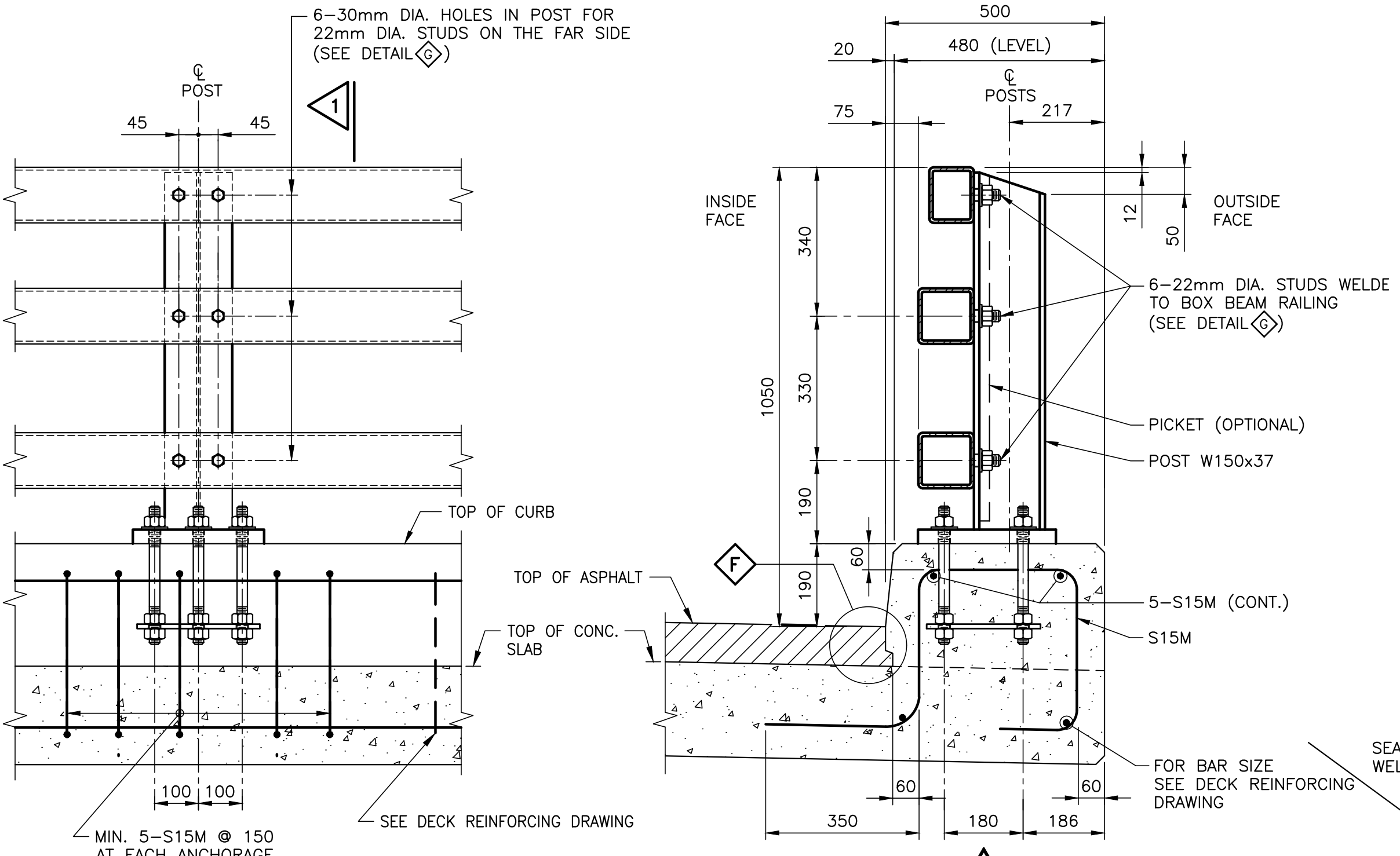
A RAIL POST ELEVATION (INSIDE FACE SHOWN)
