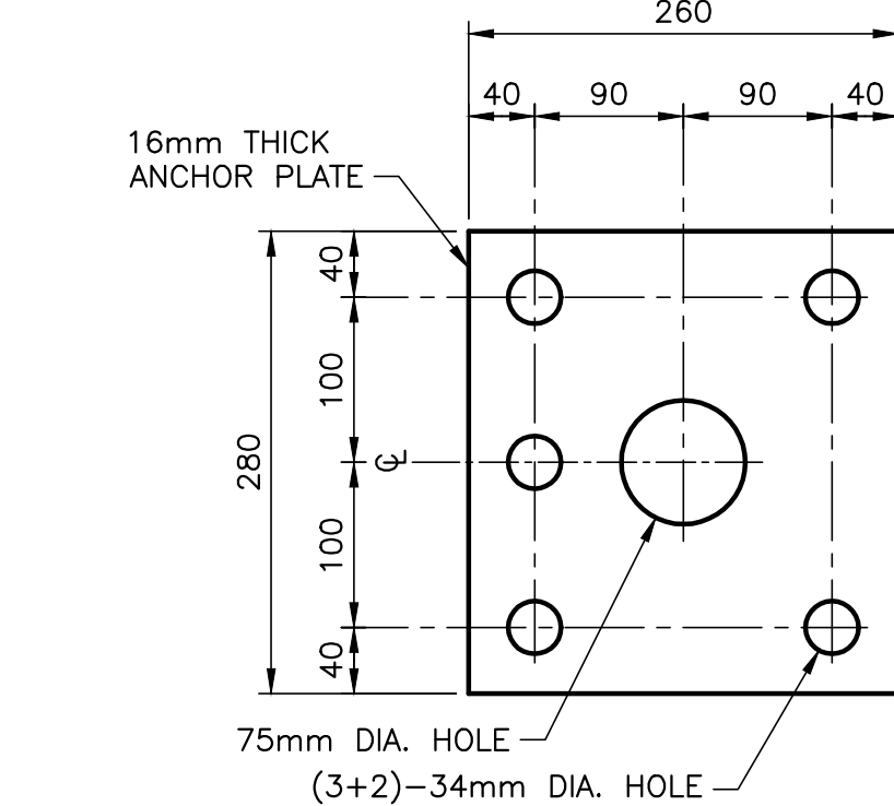
6 ANCHOR PLATE
