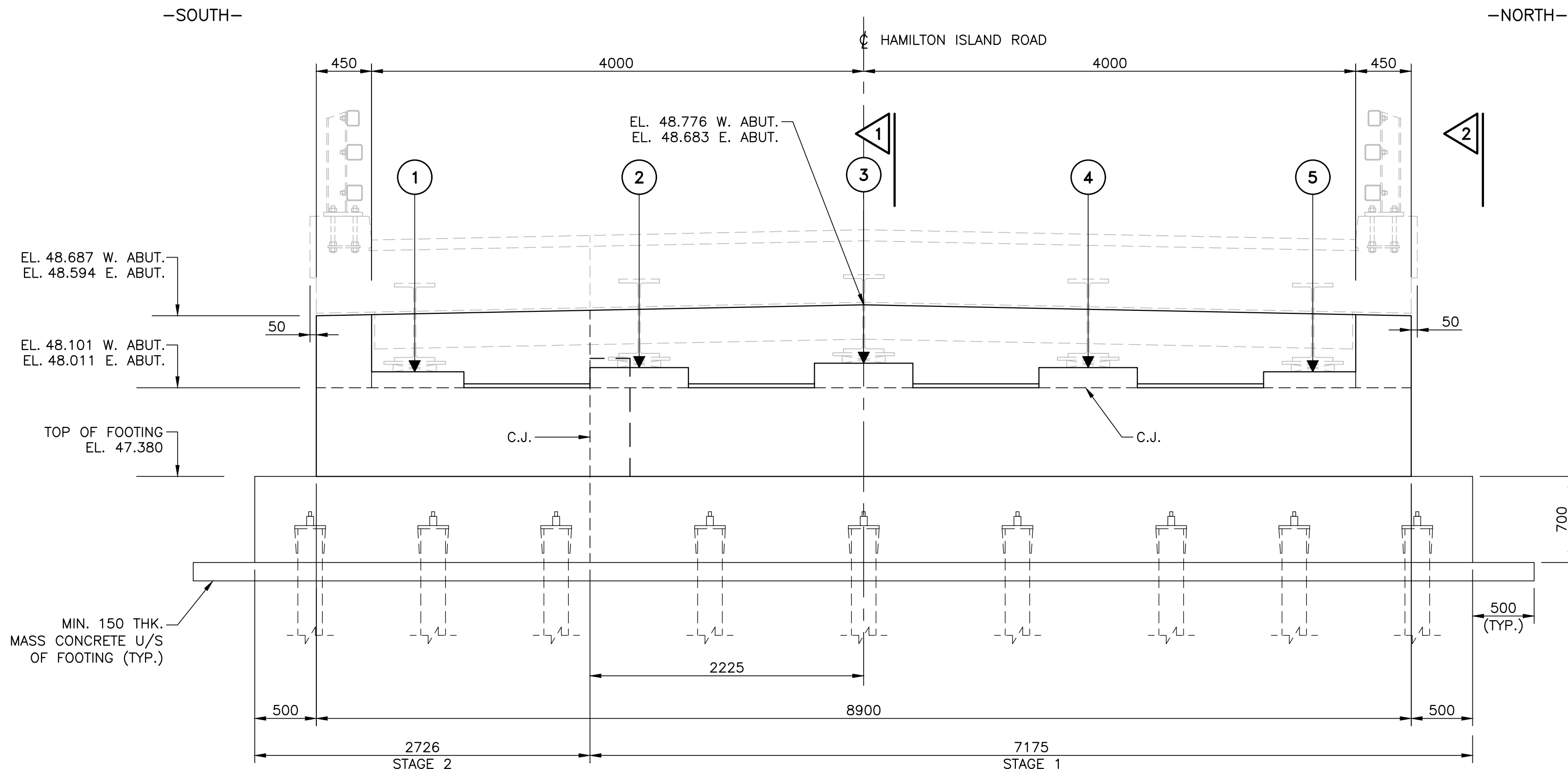
ELEVATION WEST ABUTMENT SHOWN - EAST ABUTMENT SIMILAR 1:30
