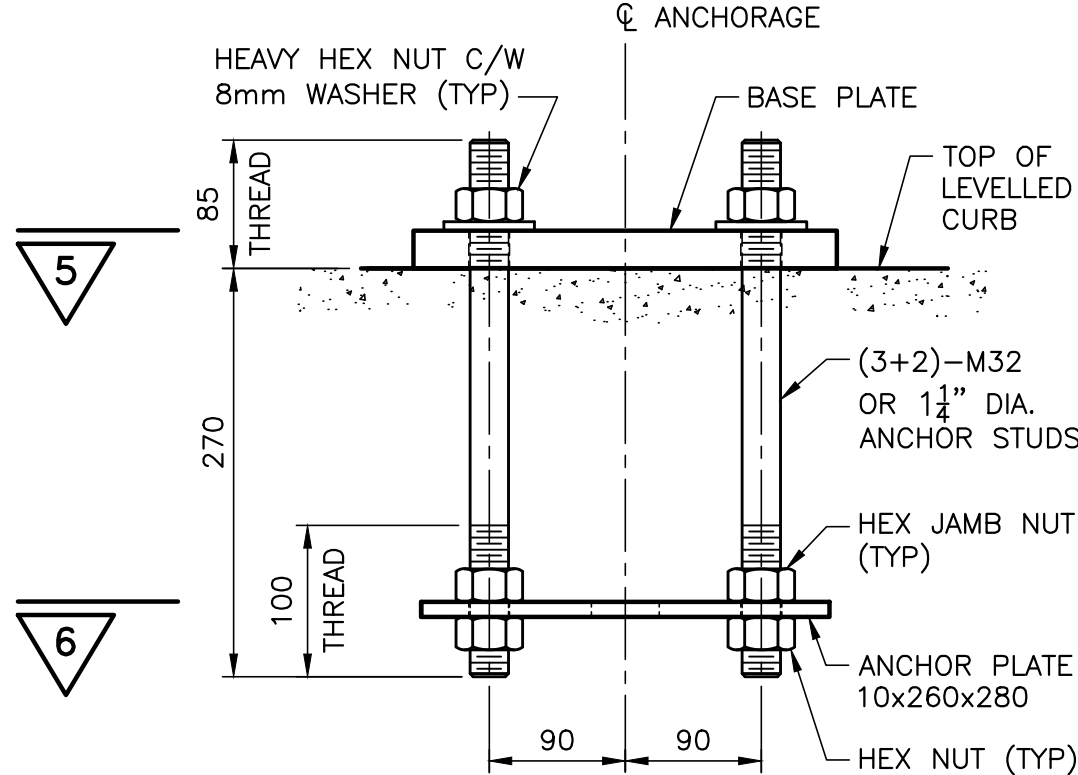
5 ANCHORAGE ASSEMBLY (SIDE SHOWN)
