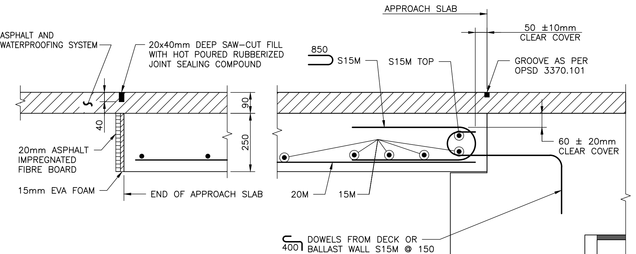
D END OF APPROACH SLAB WITH INTEGRAL/SEMI-INTEGRAL ABUTMENT SCALE 1:10
