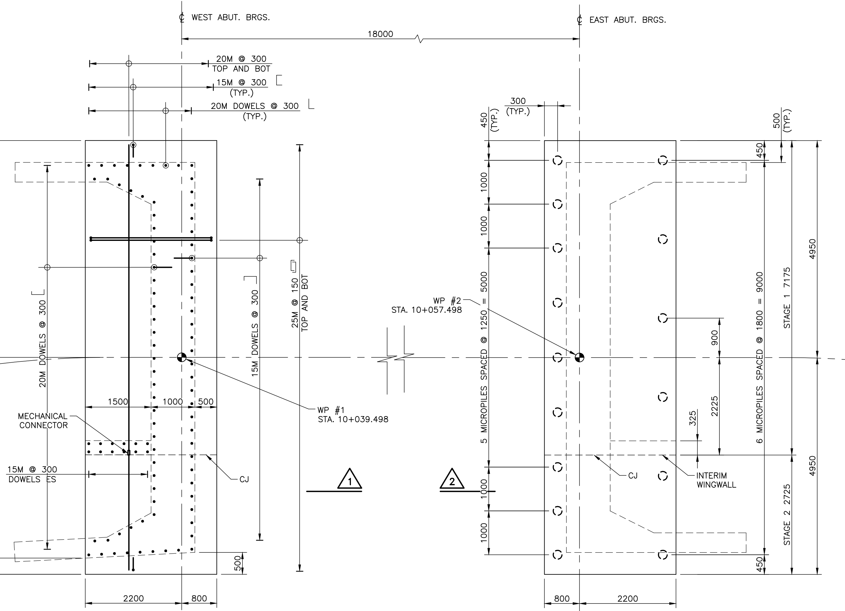
WEST ABUTMENT REINFORCING PLAN NOTE: WEST ABUTMENT SHOWN, EAST ABUTMENT SIMILAR
