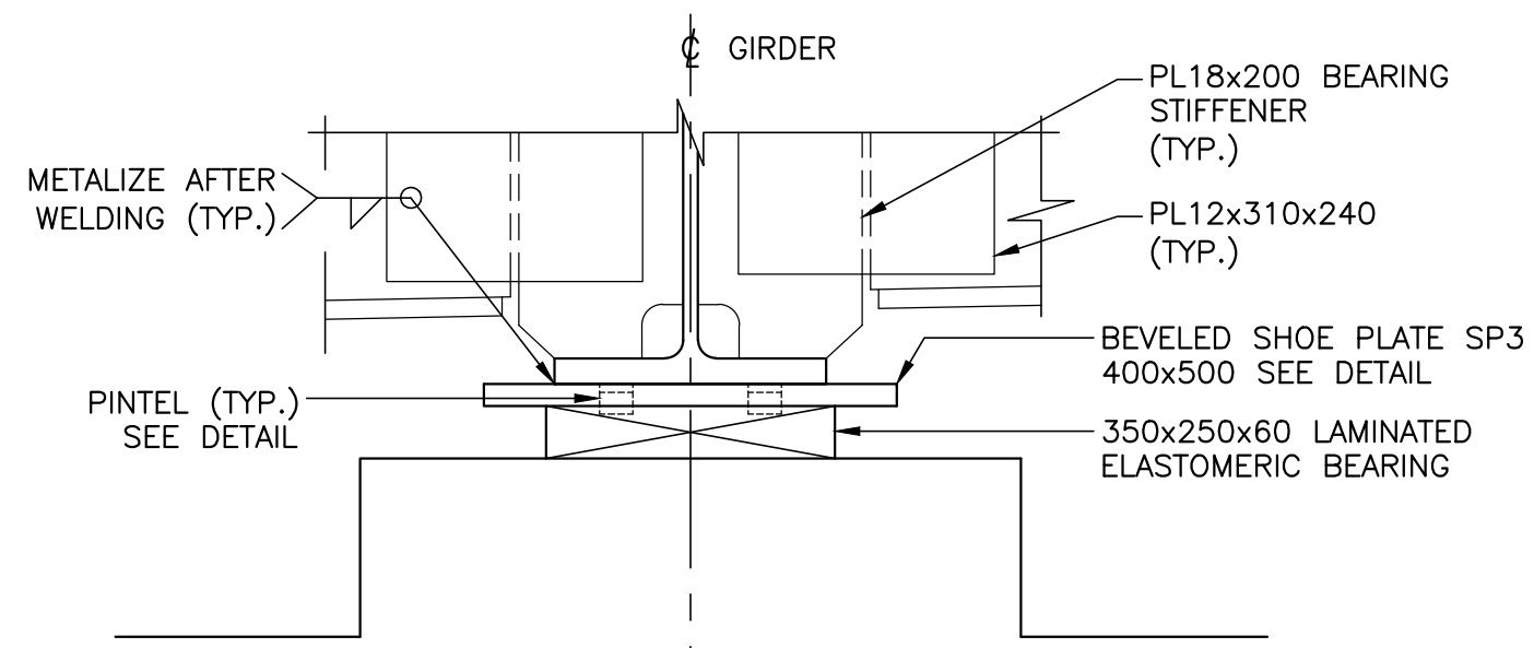
SECTION 1:10
