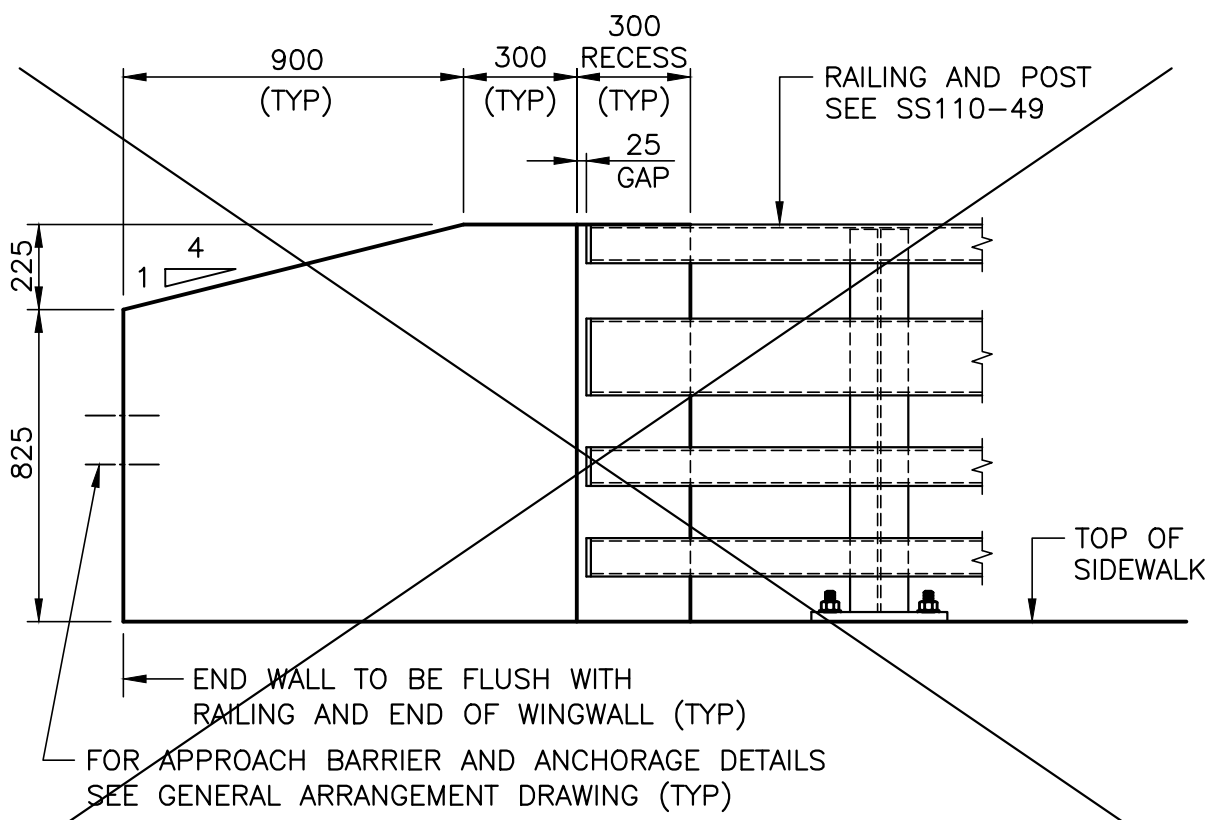
ELEVATION END WALL ON SIDEWALK (4 TUBE RAILING)
