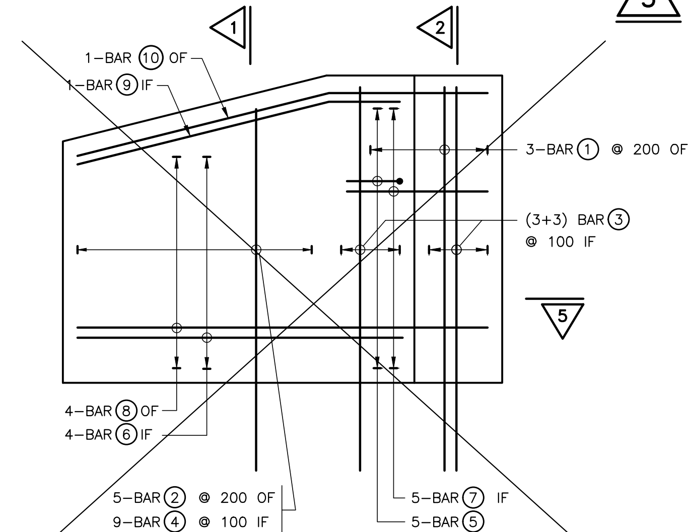
REINFORCING ARRANGEMENT - 4 TUBE RAILING END WALL ON SIDEWALK
