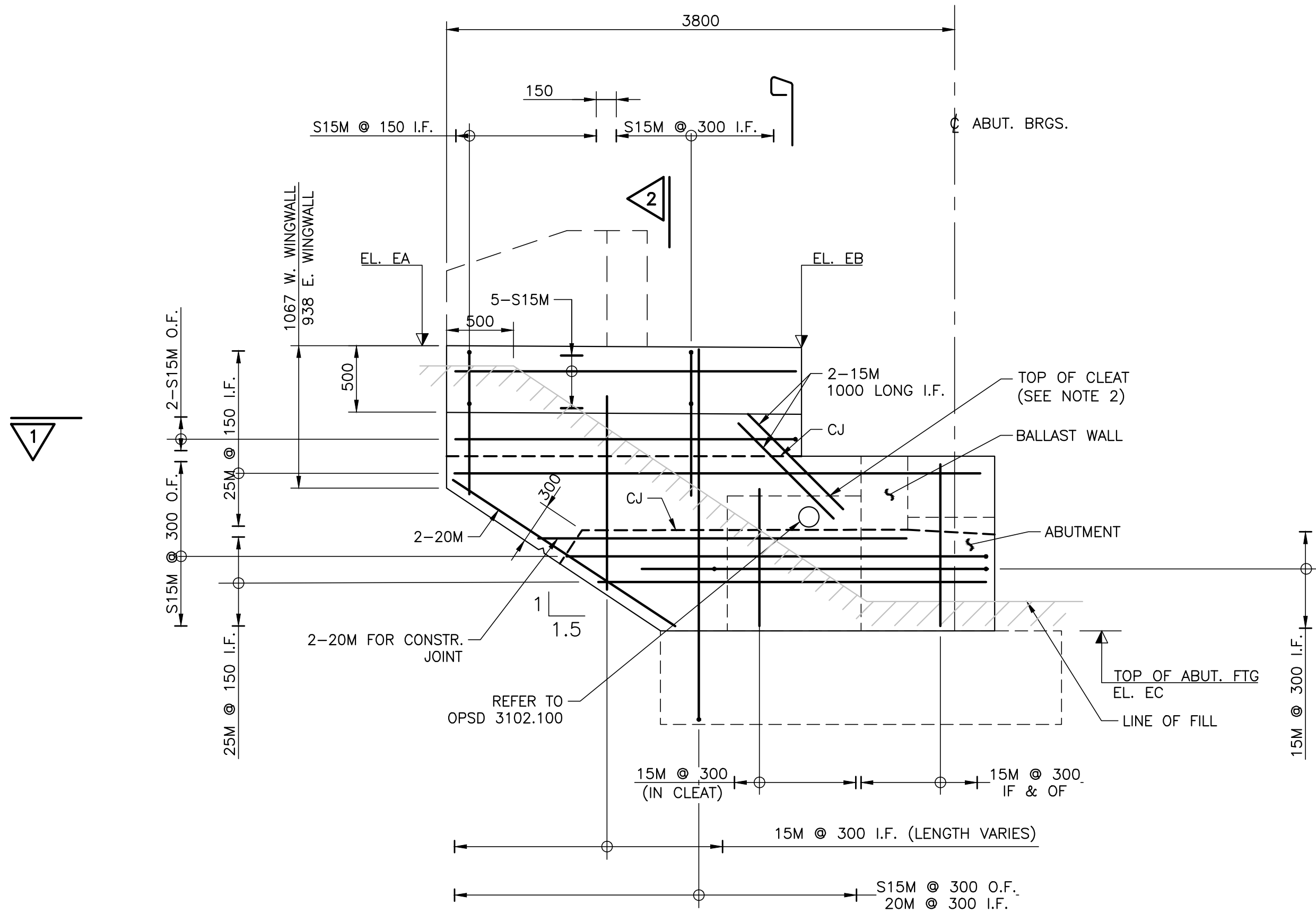
ELEVATION OF WINGWALL WITH NON-INTEGRAL ABUTMENT
