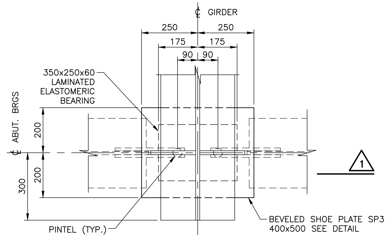
DETAIL TYPICAL ABUTMENT BEARINGS 1:10
