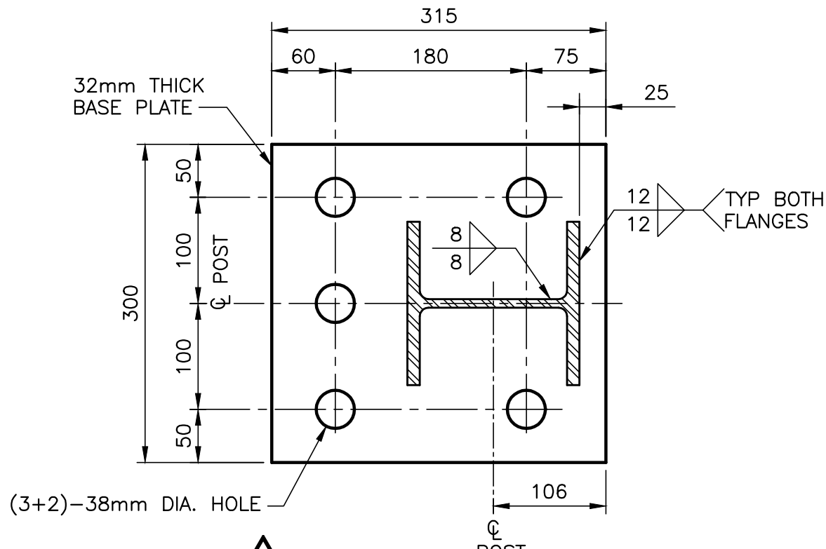
5 BASE PLATE
