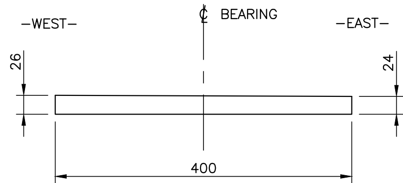
BEVELED SHOE PLATE DETAIL 1:5
