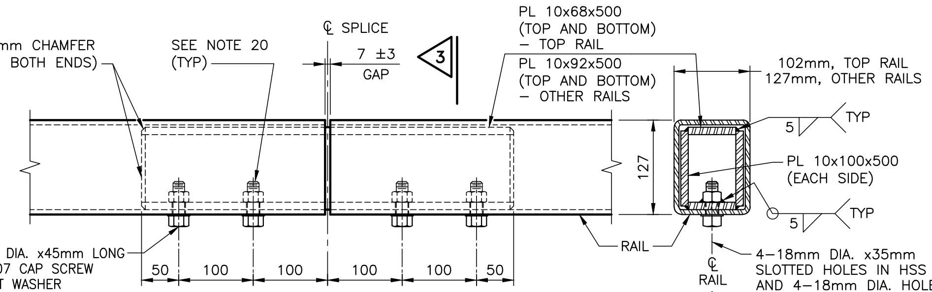
C RAIL SPLICE DETAIL
