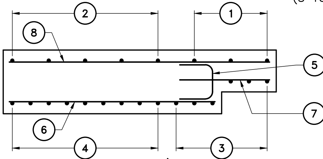
ELEVATION END WALL ON CURB (3 TUBE RAILING)
