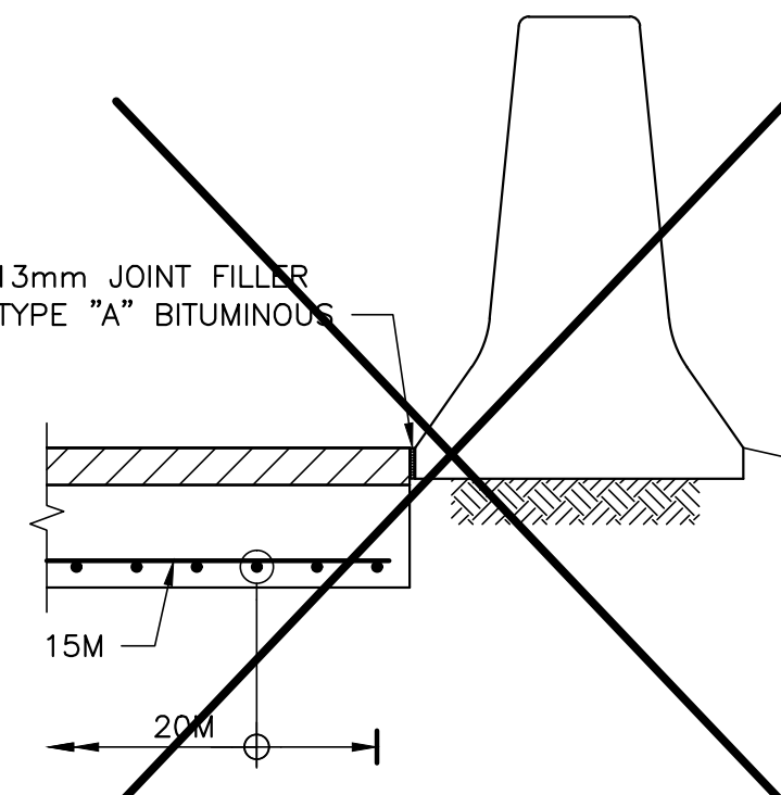
WITH ROADSIDE BARRIER
