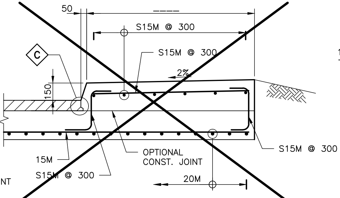
3 WITH SIDEWALK SCALE 1:20
