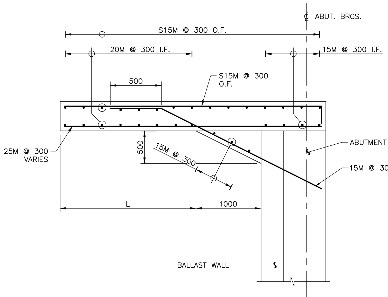
1 GENERAL WINGWALL SHOWN 1:30 (SOUTHWEST WINGWALL SIMILAR)
