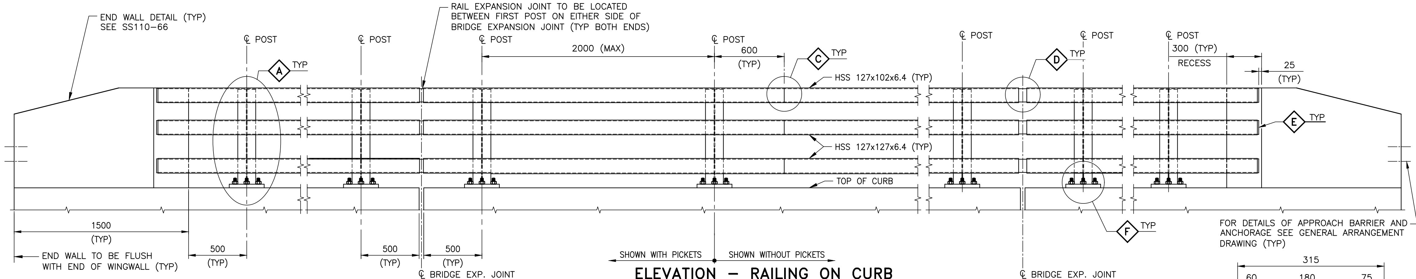
ELEVATION - RAILING ON CURB (INSIDE FACE SHOWN)
