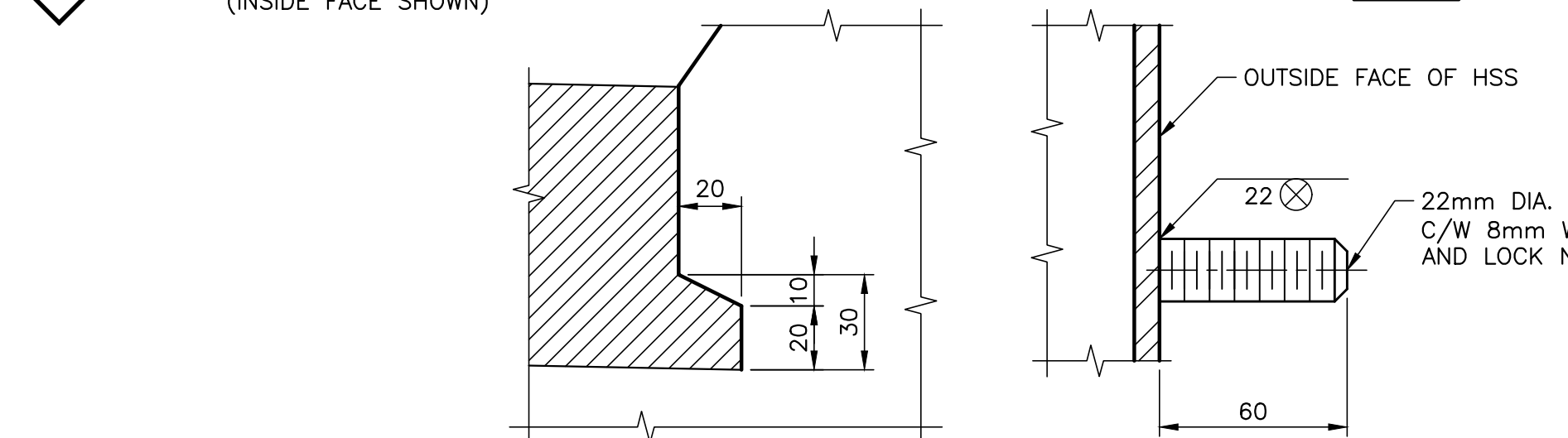
F CHASE DETAIL
