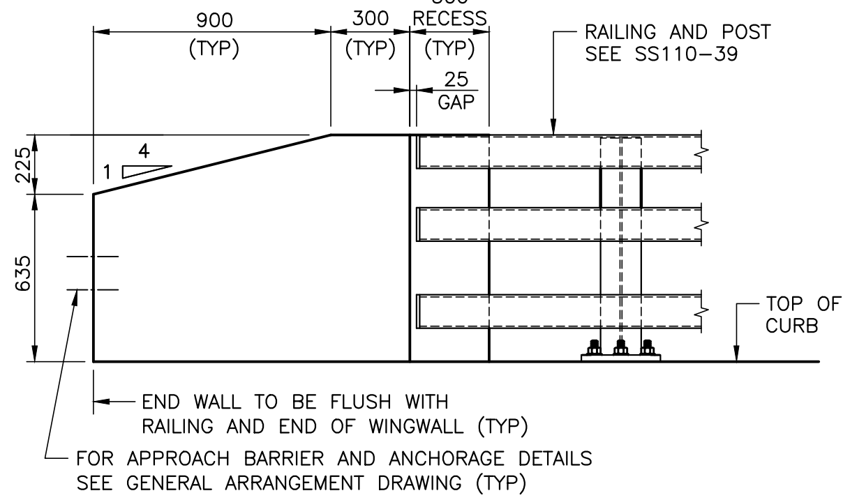
ELEVATION END WALL ON CURB (3 TUBE RAILING)
