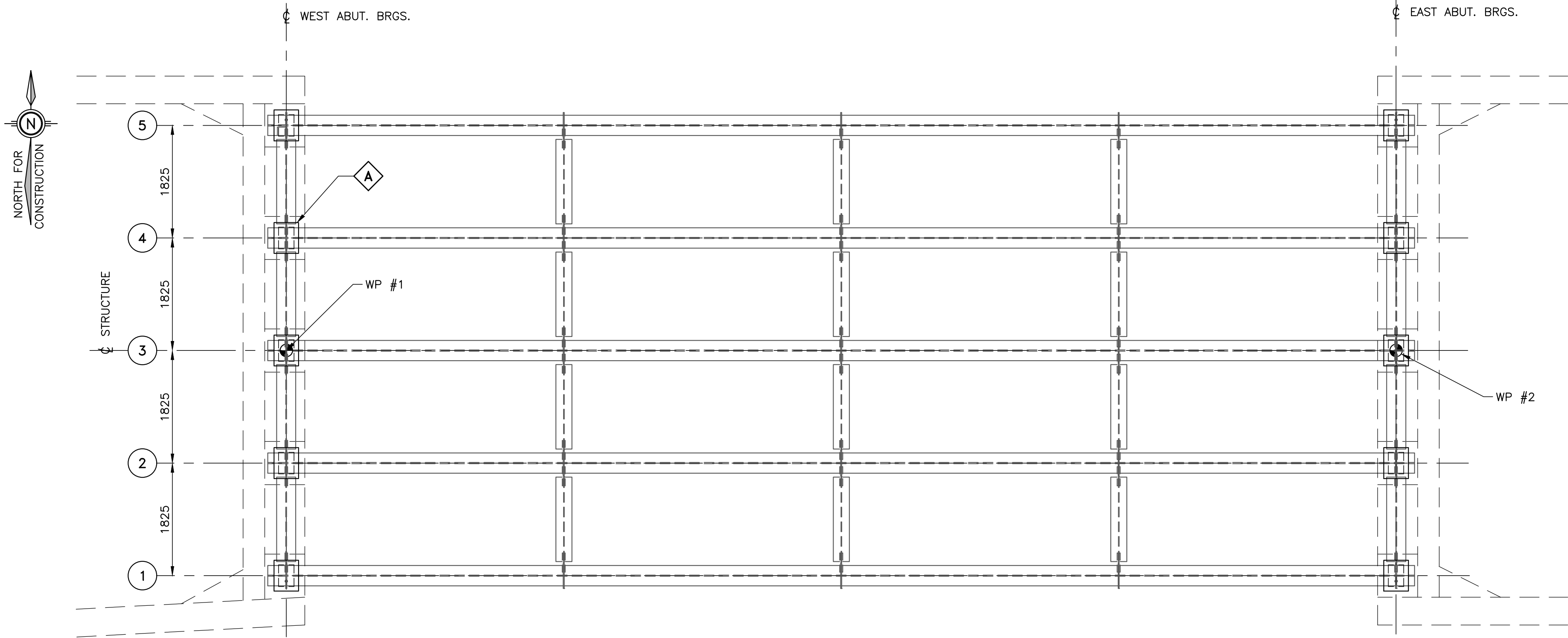
PLAN - BEARING LAYOUT 1:50
