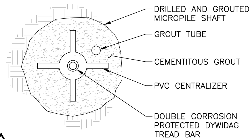
SECTION 4 1:5
