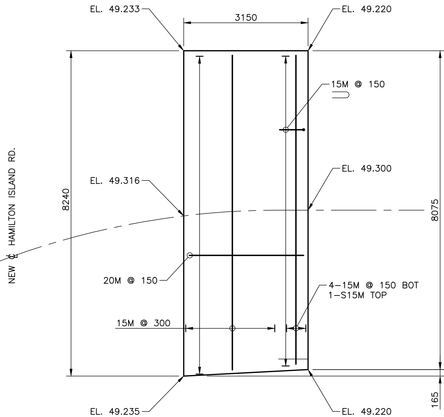
PLAN - WEST APPROACH SLAB 1:60
