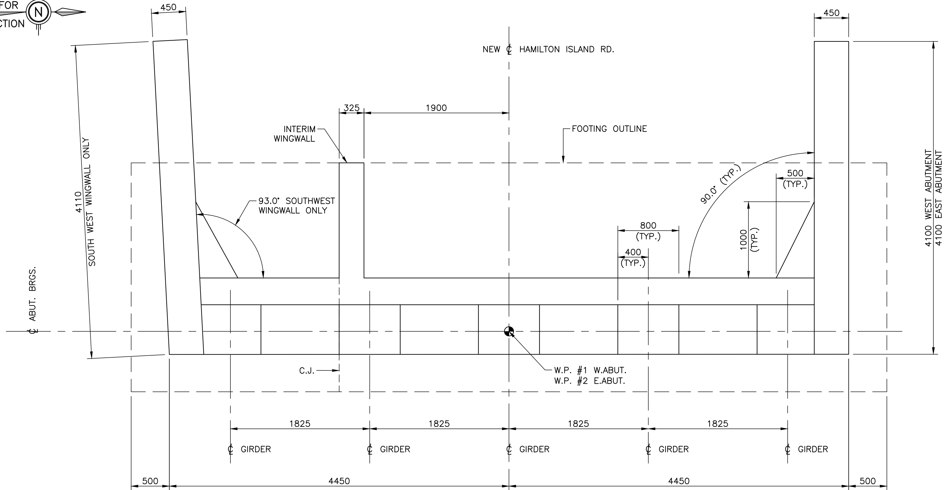
PLAN WEST ABUTMENT SHOWN - EAST ABUTMENT SIMILAR 1:30
