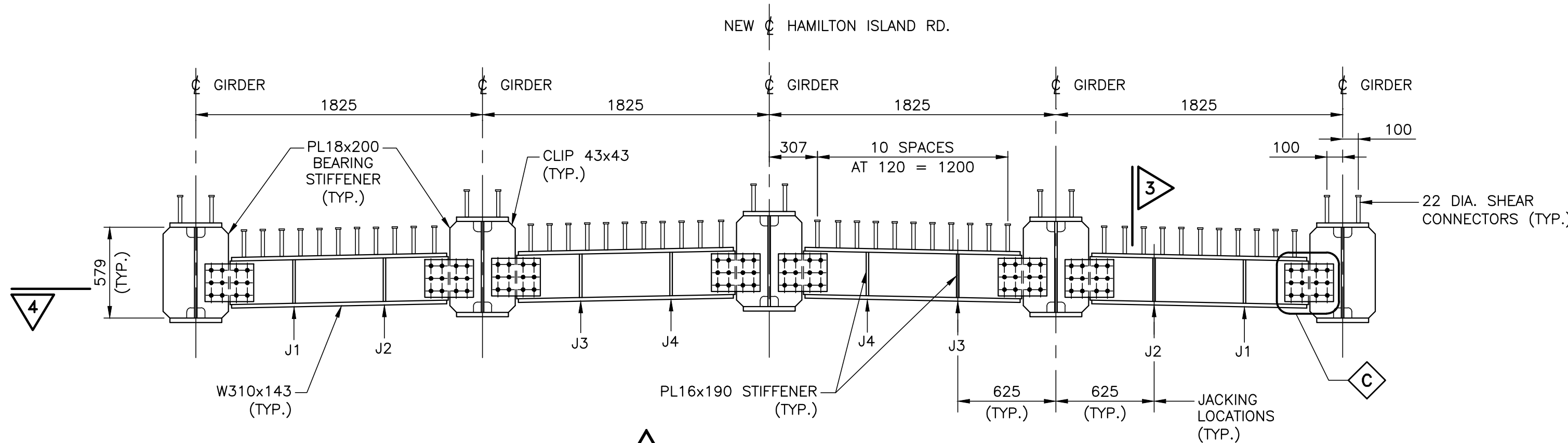
1 BEARING DIAPHRAGM 1:25 DWG. 14
