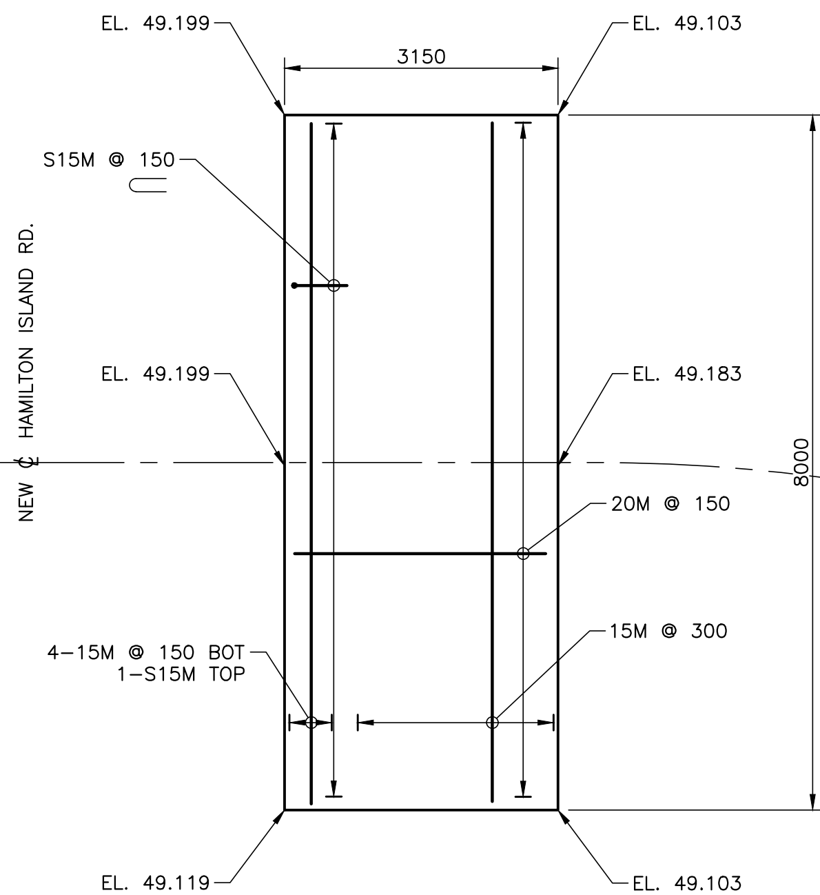
PLAN - EAST APPROACH SLAB 1:60
