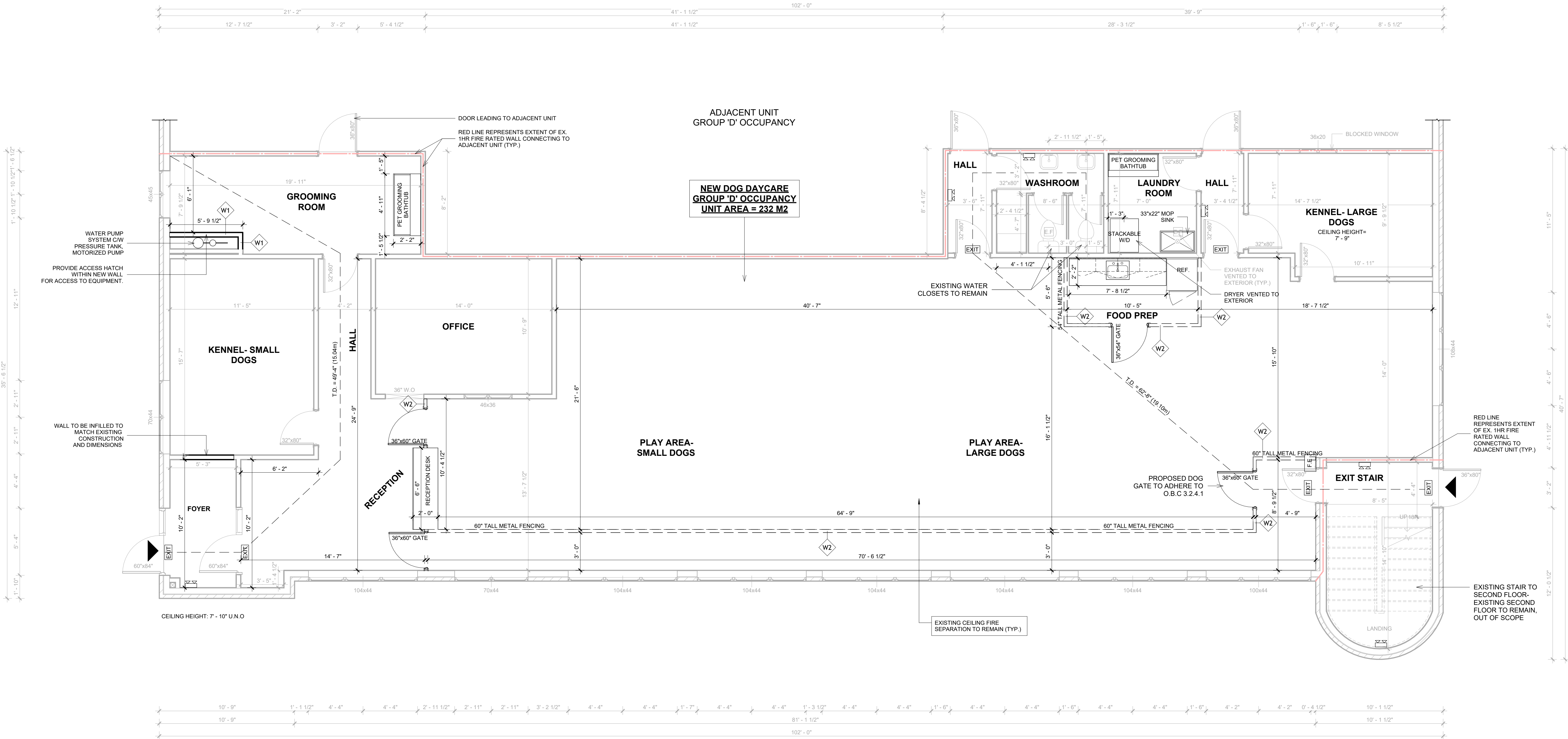
1 PROPOSED MAIN FLOORPLAN 1/4" = 1'-0"
