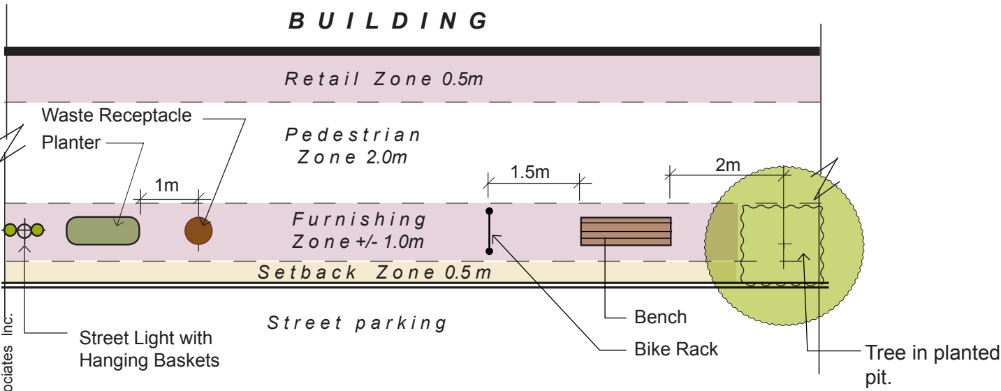
Furnishing Placement Guidelines: Sidewalk +/- 4.0m wide
