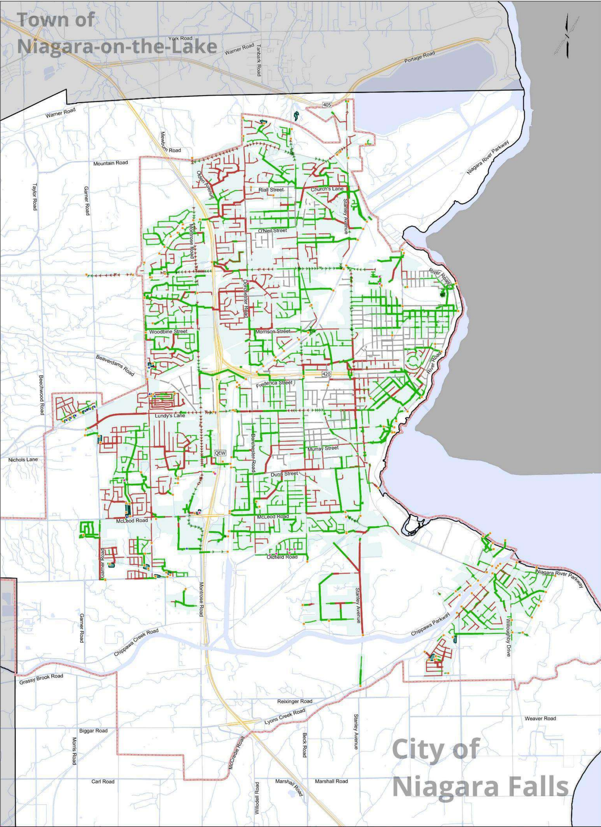
Figure 5-2 Existing System Performance under 100-Year Design Storm
