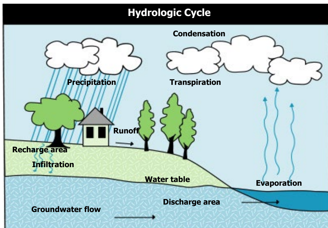
Figure 3-1: Hydrologic Cycle
