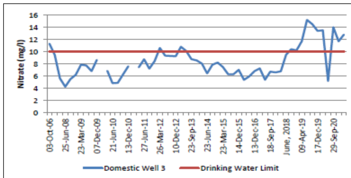
Figure 5-7: Nitrate Levels in Domestic Well #3
