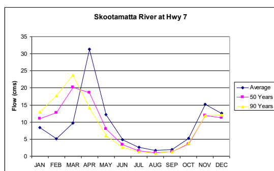
Figure 7-2: Skootamatta River at Hwy 7 Flows (m³/s)
