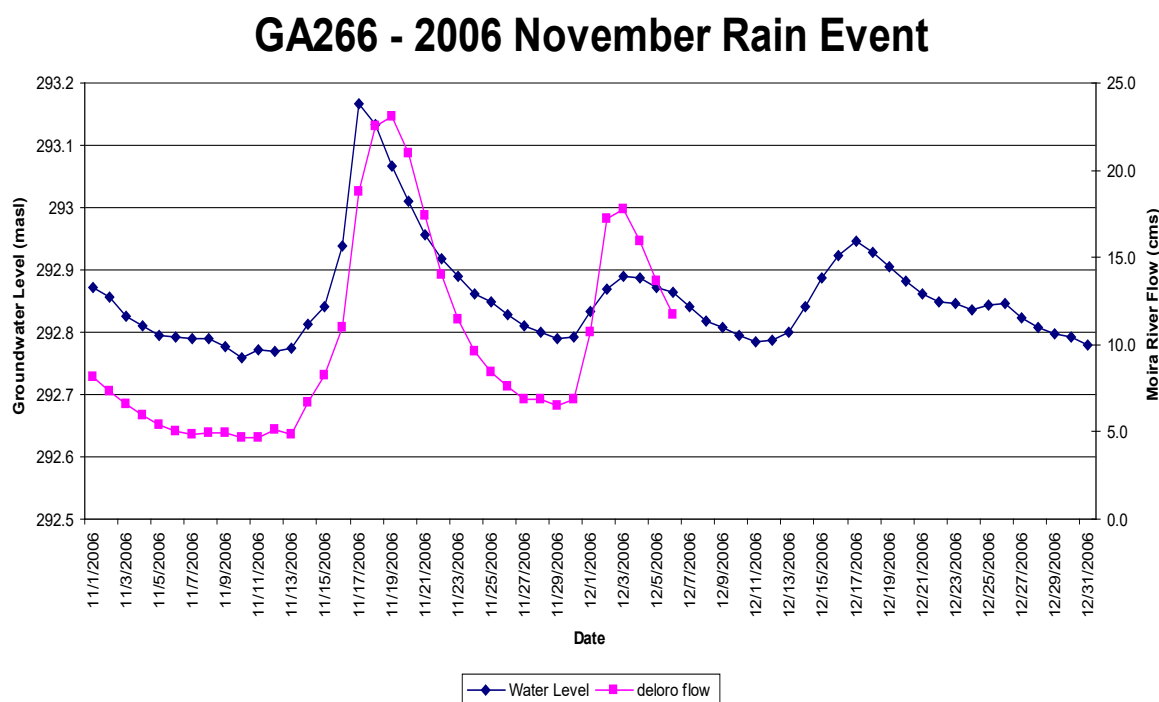
Figure 5-3: Ground and Surface Water Hydrographs November 2006
