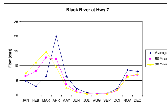
Figure 7-3: Black River at Hwy 7 Flows (m³/s)
