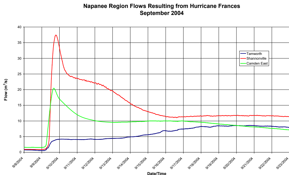
Figure 3-6: Napanee Region Hydrographs
