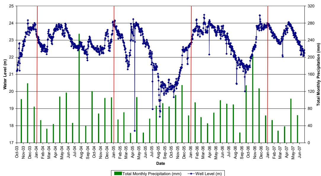
Figure 5-5: Deloro Municipal Well Hydrograph with Monthly Precipitation
