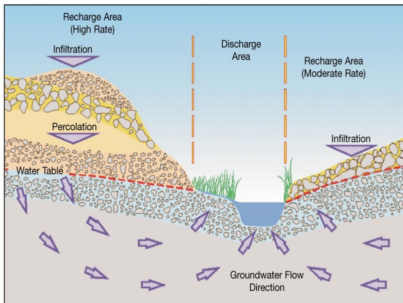
Figure 4-2: Groundwater Recharge
