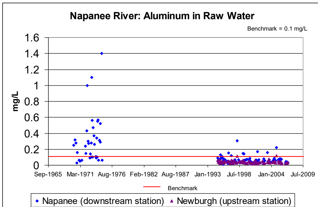
Figure 6-3: Concentrations of Aluminum in Raw Water Samples
