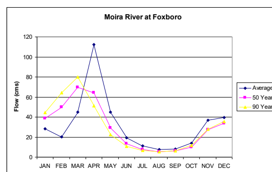
Figure 7-4: Moira River at Foxboro Flows (m³/s)
