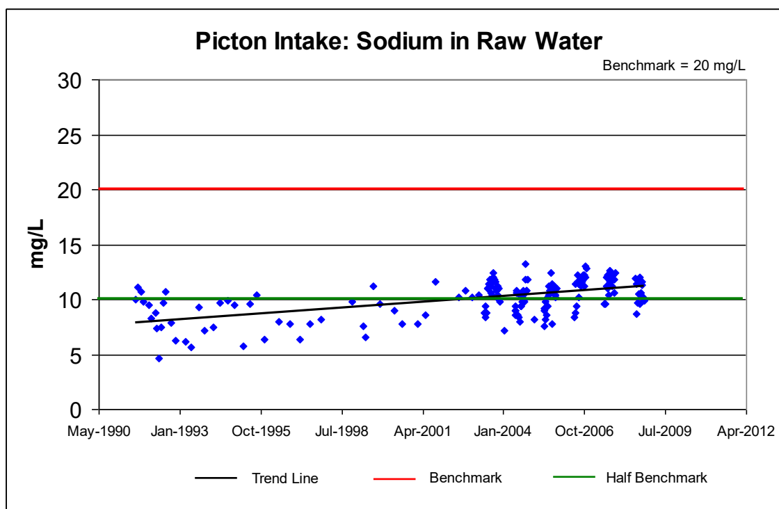
Figure 6-2: Sodium Time Series
