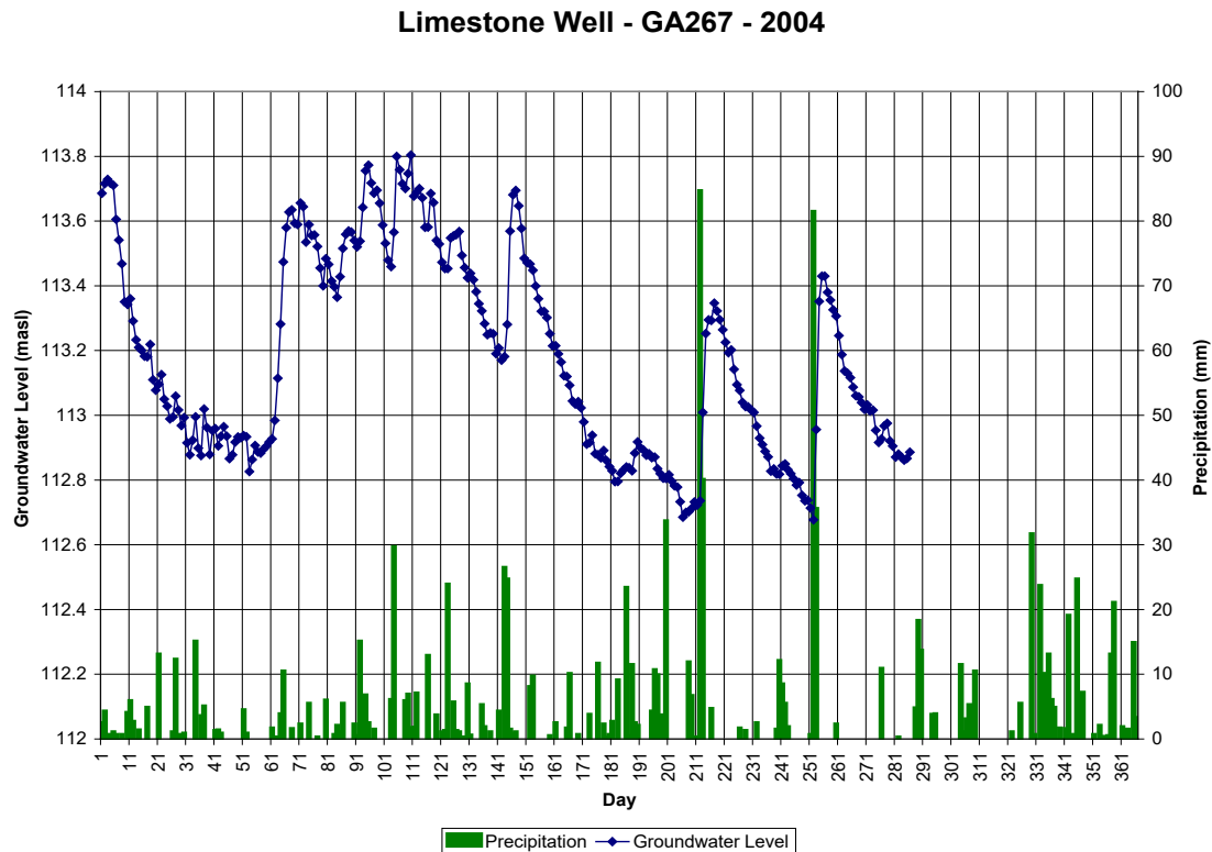
Figure 5-2: Groundwater Hydrograph Paleozoic Aquifer
