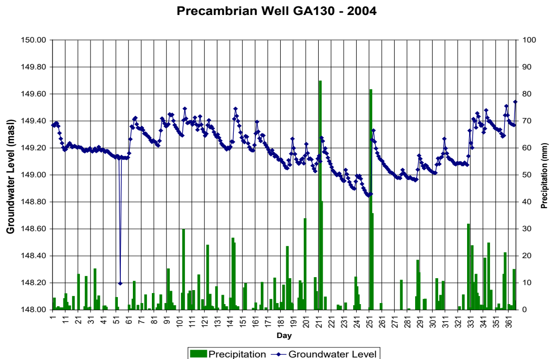
Figure 5-1: Groundwater Hydrograph Precambrian Aquifer
