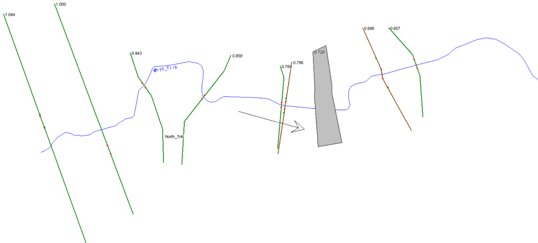
HEC-RAS Model Schematic – Post-Development
