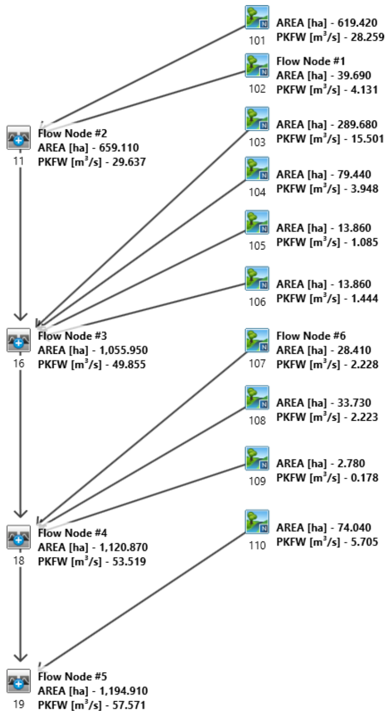
Figure E.1: VO5 Model Schematic – Floodplain Drainage Area
